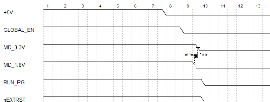
Figure 5-2 Power-down sequencing
