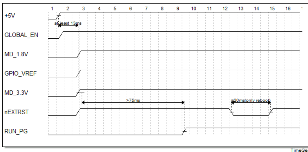
Figure 5-1 Power-Up sequencing
