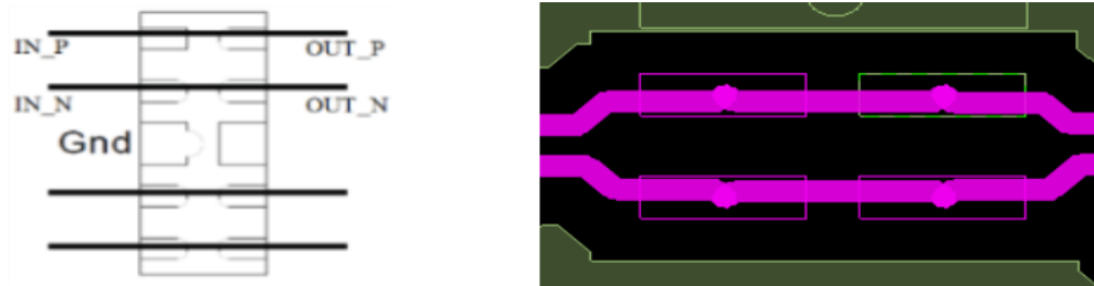
Figure 8-17. ESD Void
