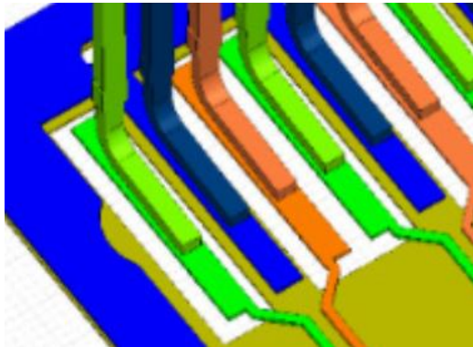
Figure 8-20. Connector Voiding
